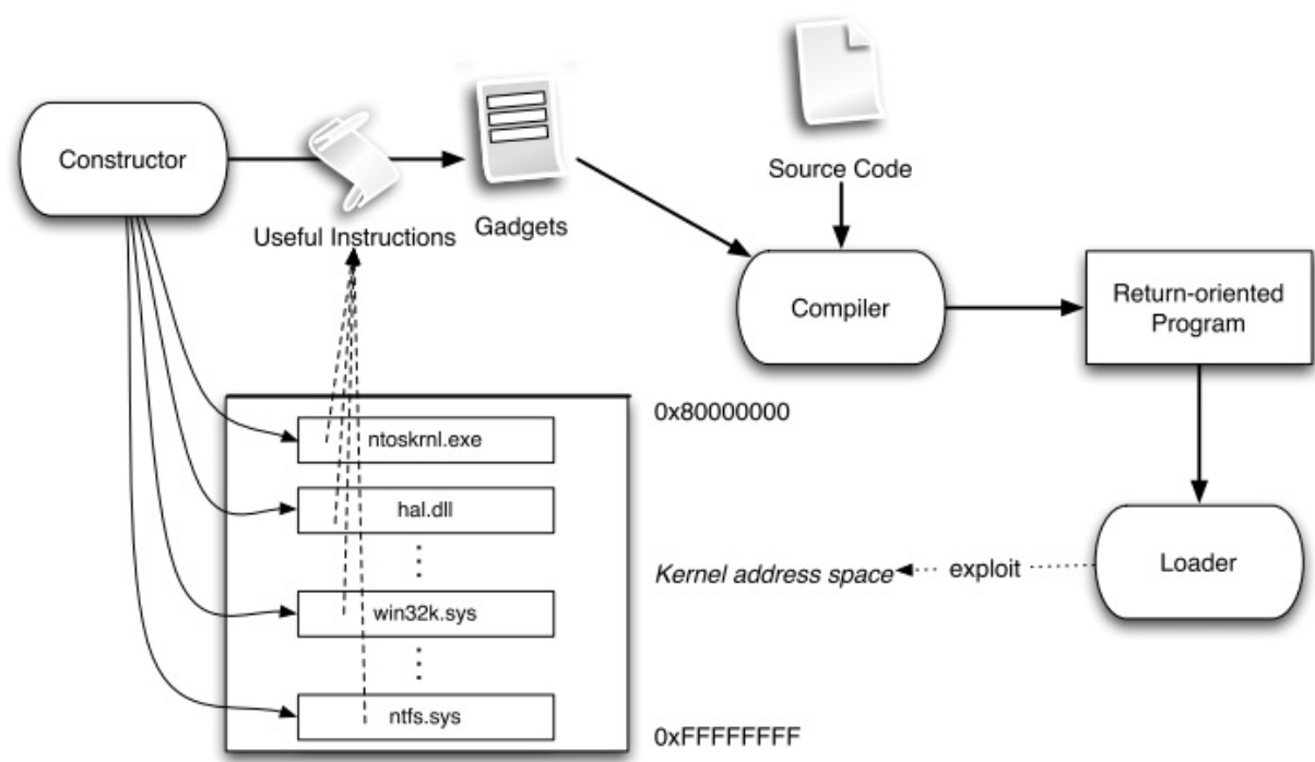
Figure 2: Schematic system overview
