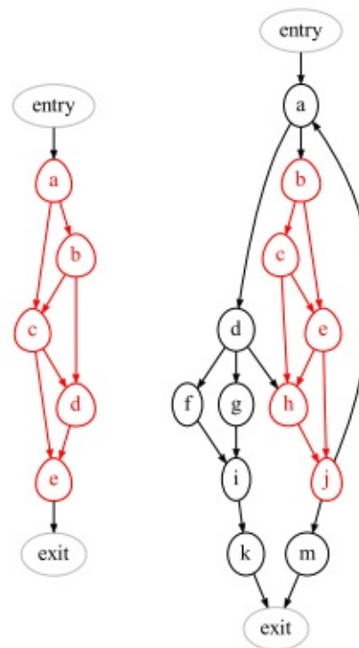
Figure 2: An example of ACFG matching. The graph on the left ( M , a malware sample) is matched as a subgraph of the graph on the right ( P_{sg} , the malware embedded inside a benign program), i.e, M = (a, b, c, d, e) \cong P_{sg} = (b, c, e, h, j) , where M \cong P_{sg} denotes that M is isomorphic [29] to P_{sg} .
