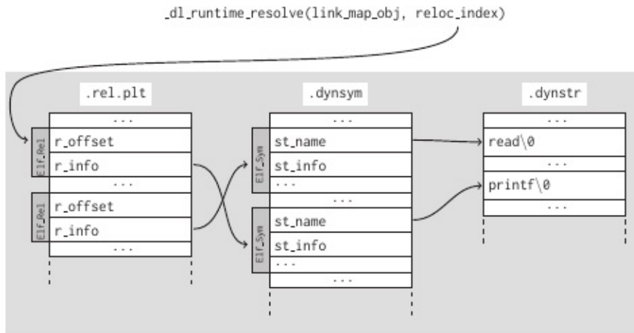
Figure 1: The relationship between data structures involved in symbol resolution (without symbol versioning). Shaded background means read only memory.
