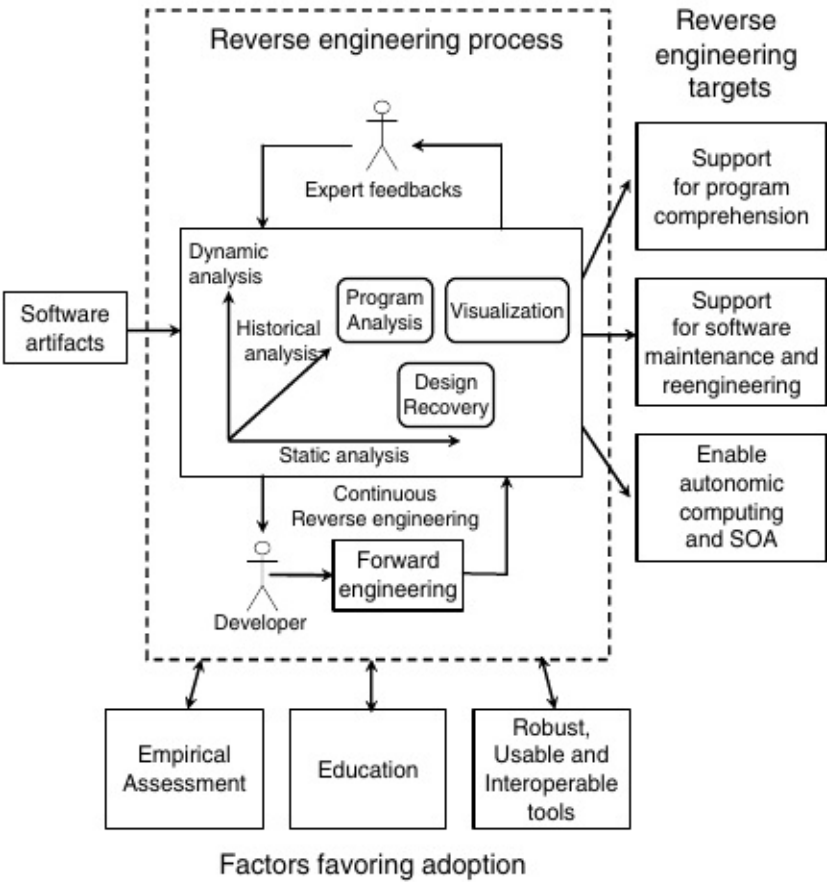
Figure 5. The role of reverse engineering
