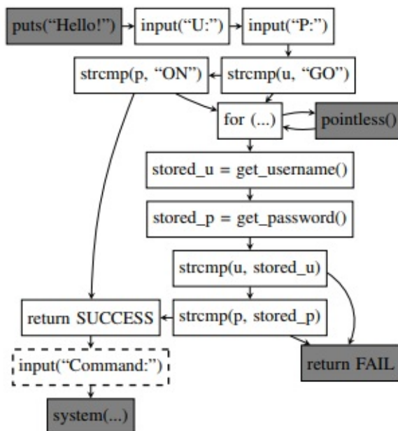
Fig. 1: Fimalice’s CFG for the example. The darkened nodes are excluded from the authentication slice.
