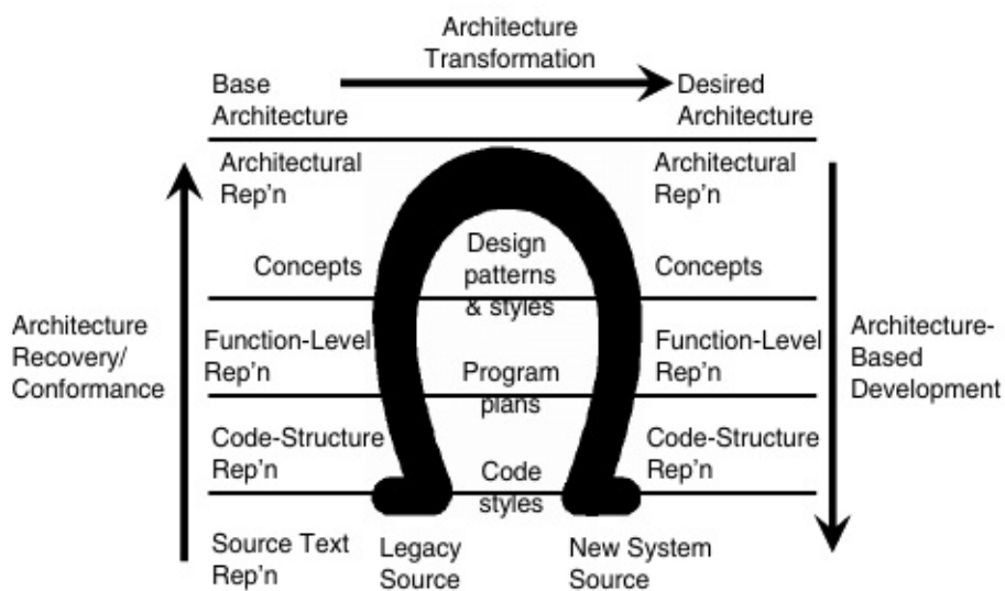
Figure 2. Architecture Reengineering: The Horseshoe model [64]
