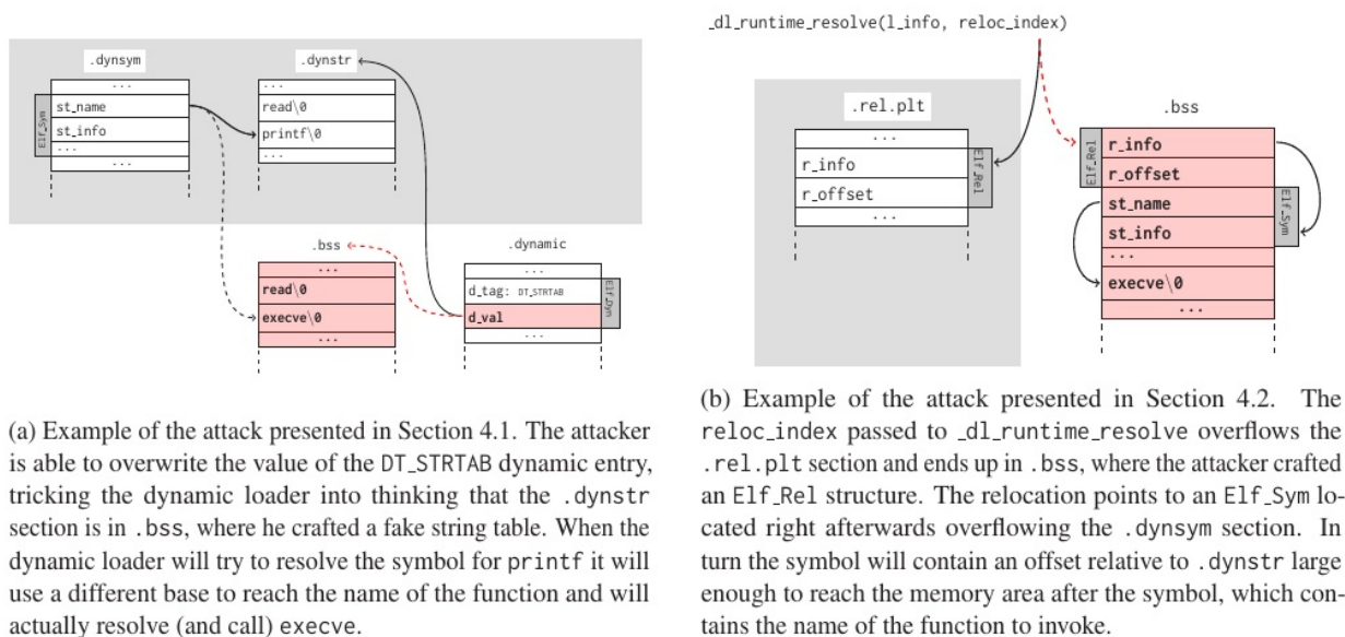
Figure 2: Illustration of some of the presented attacks. Shaded background means read only memory, white background means writeable memory and bold or red means data crafted by the attacker.
