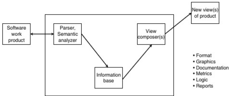
Figure 1. Reverse engineering tools architecture [28]
