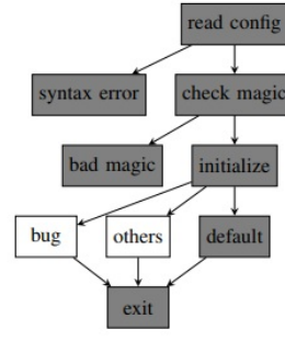
Fig. 3. The nodes found by the fuzzer, supplemented with the result of the first Driller run.
