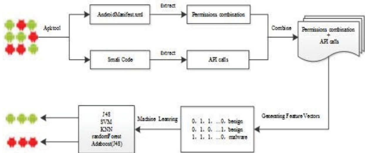
Fig. 1 The malware detection framework
