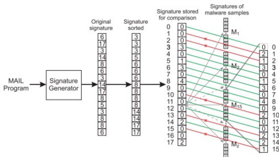
Figure 4: A successful SWOD signature matching.
