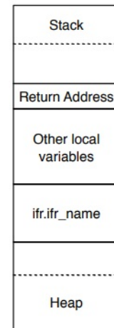
Figure 2: Memory Diagram
