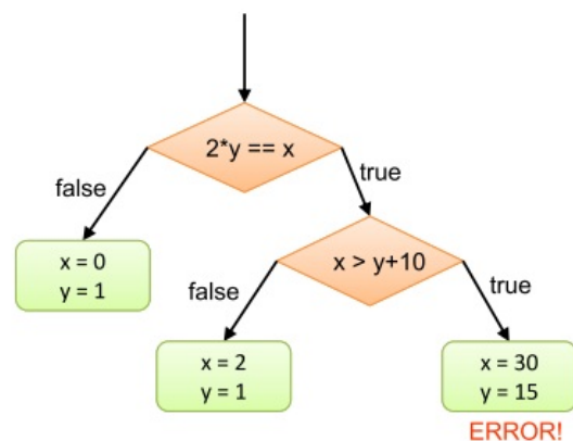
Figure 2. Execution tree for the example in Figure 1.
