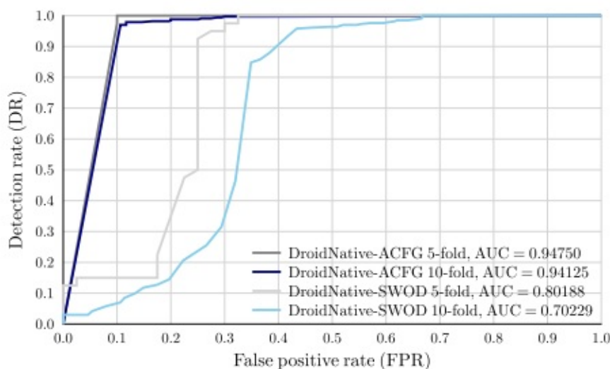
Figure 5: ROC graph plots of DroidNative's ACFG and SWOD
