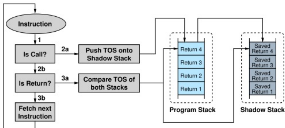
Figure 3: Our high-level approach
