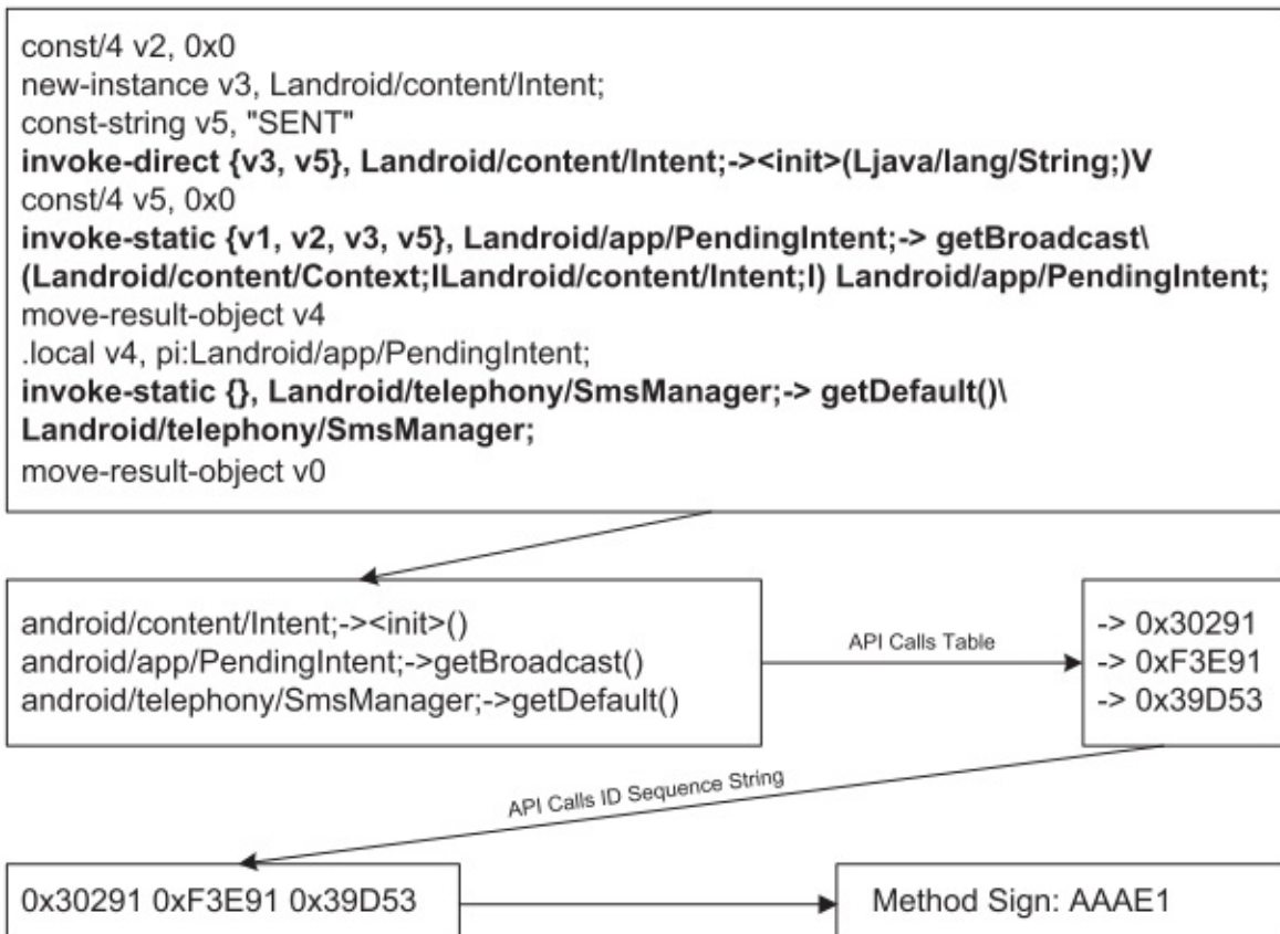
Fig. 2. The Process of Lev3 Signature Generation
