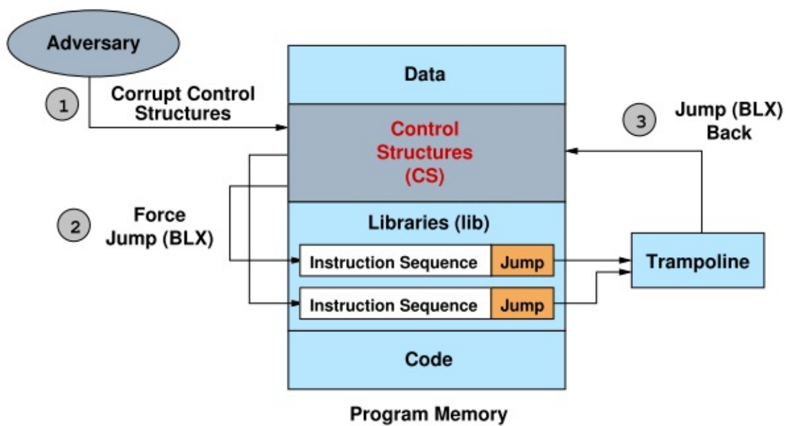
Figure 1: Return-oriented programming without returns
