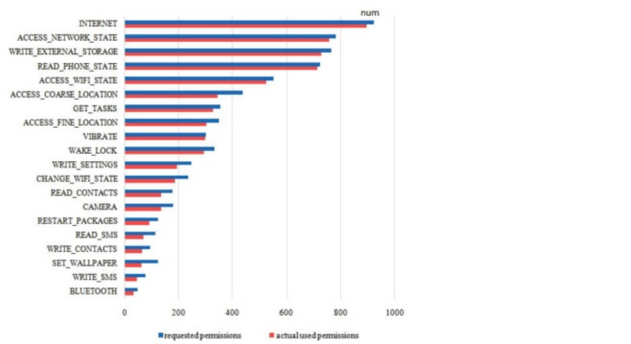
Fig. 3 Top 20 permissions that requested and actually used among benign samples
