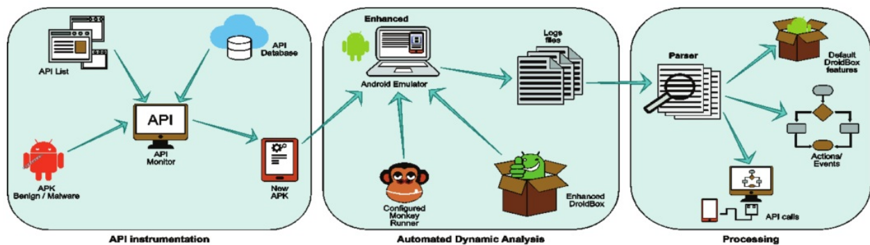
Fig. 1. DynaLog architecture
