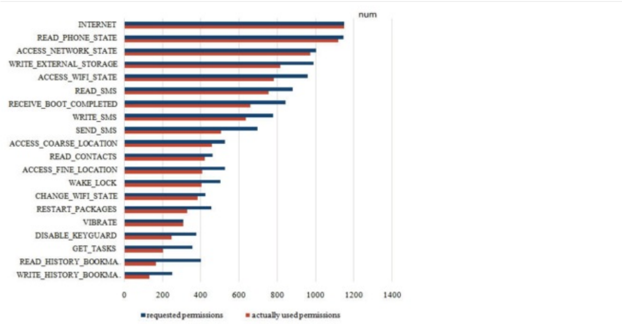
Fig. 2 Top 20 permissions that requested and actually used among malware samples
