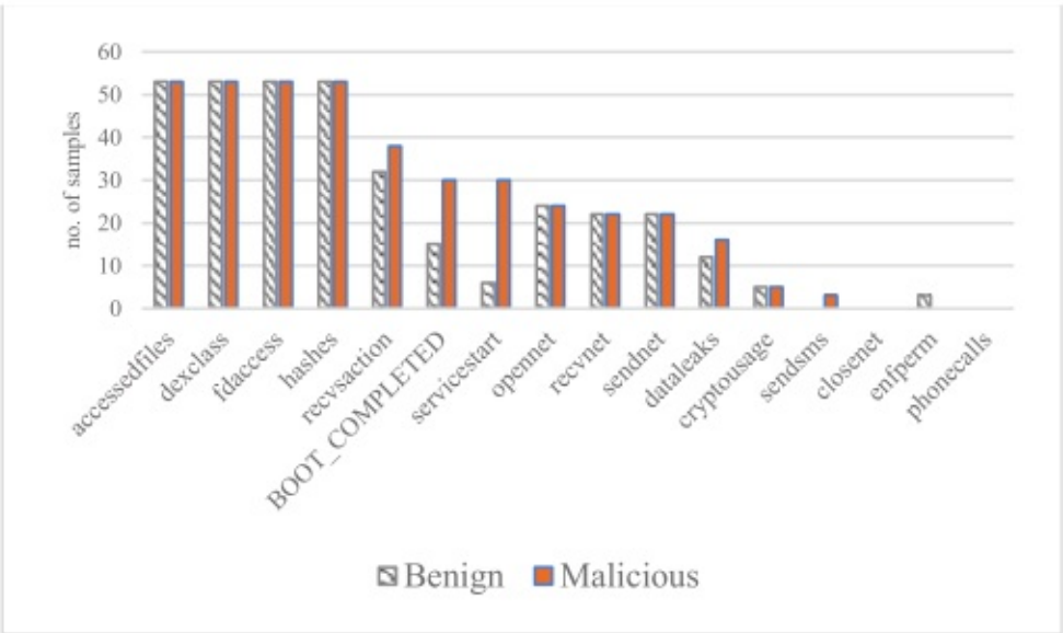
Fig 3. Behaviour logs from 106 APKs using DynaLog configured to enable only the default DroidBox features.
