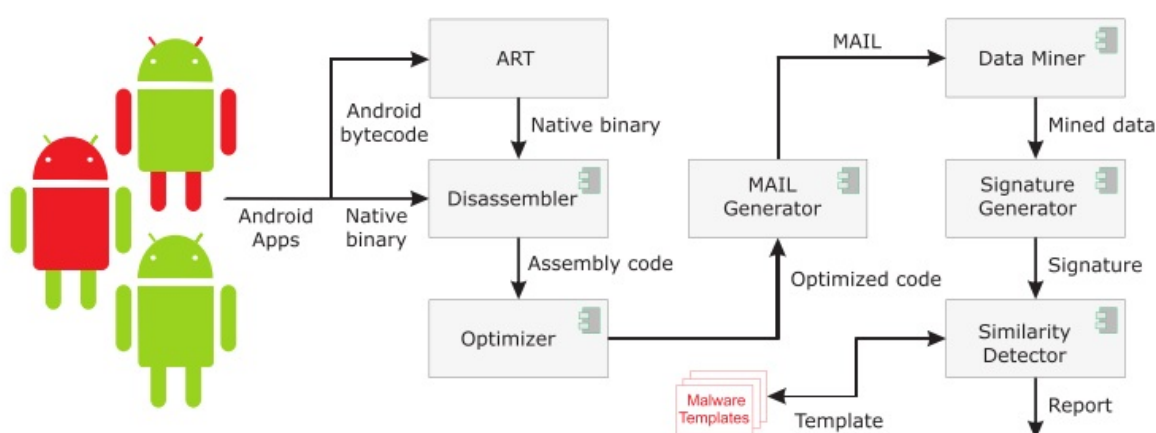
Figure 1: Overview of DroidNative.
