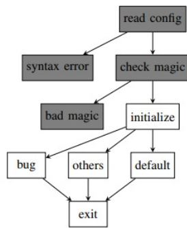
Fig. 1. The nodes initially found by the fuzzer.
