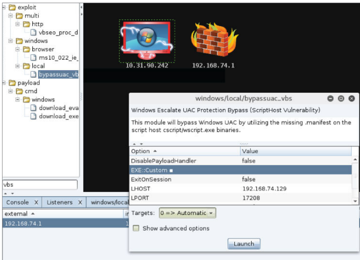
Figure 4.14: Exploiting a vulnerability in the ScriptHost to escalate to the system.
